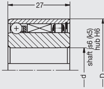
with bearing
