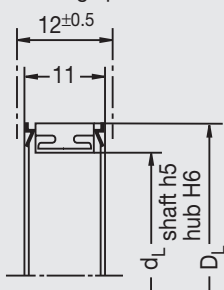
Mounting space
